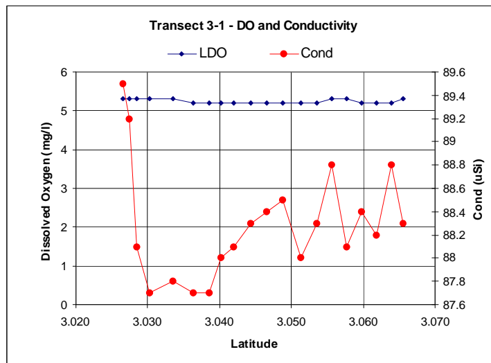
Figure T-1: Run 1 – Unit 5 at 37% Gate
