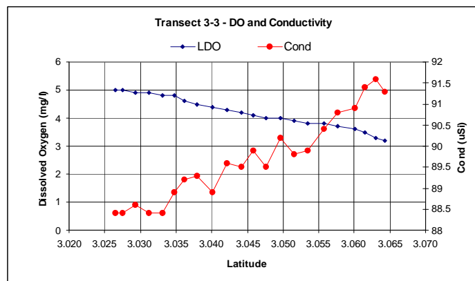
Figure T-3: Run 3 – Unit 1 at 80% Gate (ABV, Closed) and Unit 5 at 37% Gate
